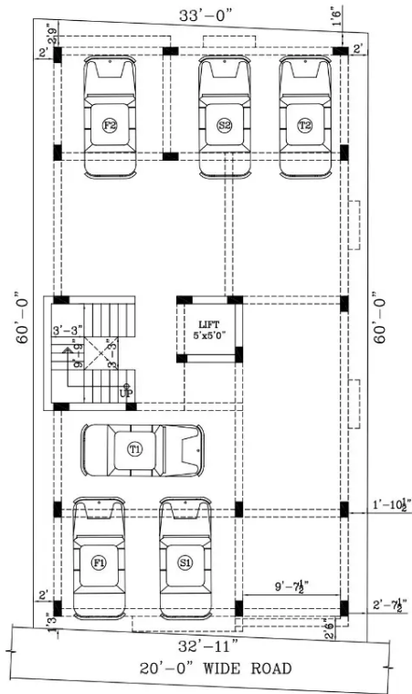
SITE CUM GROUND FLOOR PLAN
