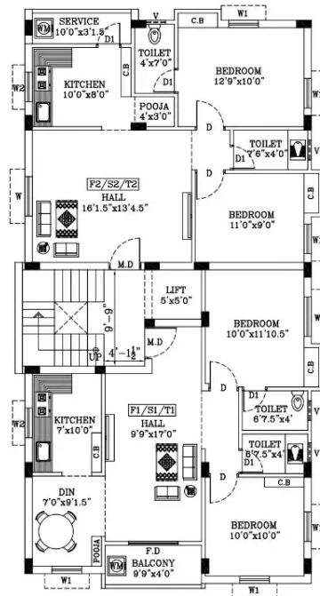
TYPICAL FLOOR PLAN (FIRST, SECOND & THIRD)
