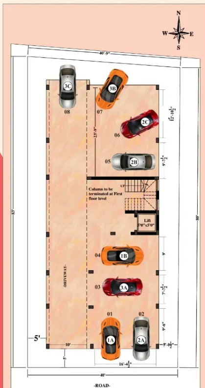
STILT FLOOR PLAN
