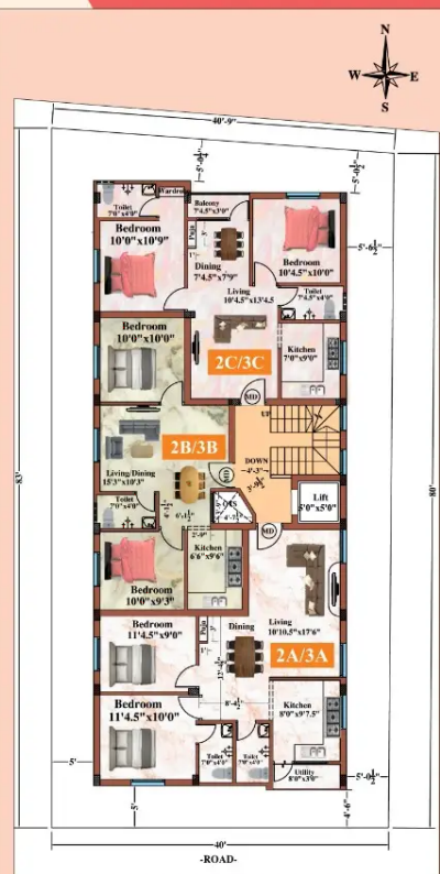
TYPICAL FLOOR PLAN (II) (III)
