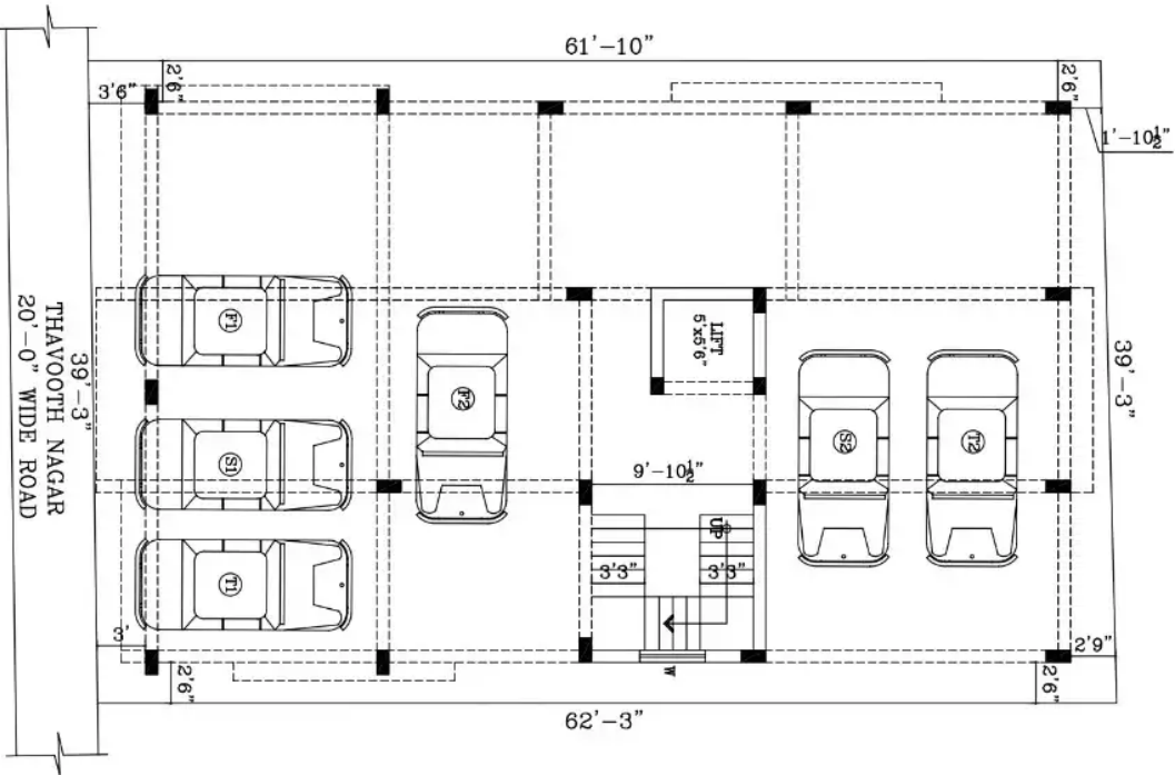
SITE CUM GROUND FLOOR PLAN
