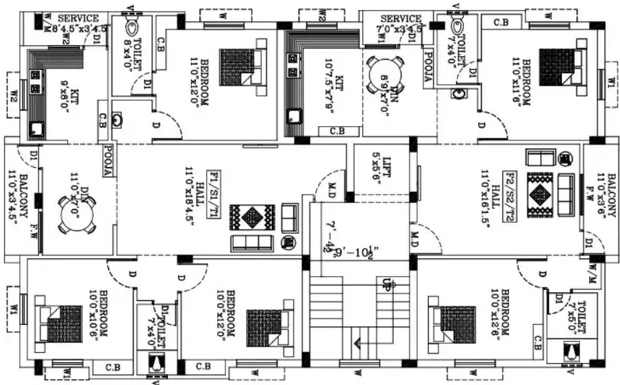
TYPICAL FLOOR PLAN (FIRST, SECOND & THIRD)
