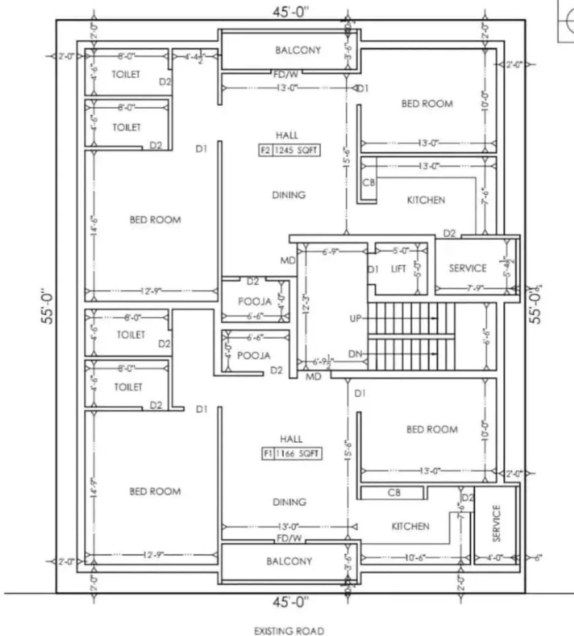
FIRST, SECOND & THIRD TYPICAL FLOOR PLAN.
