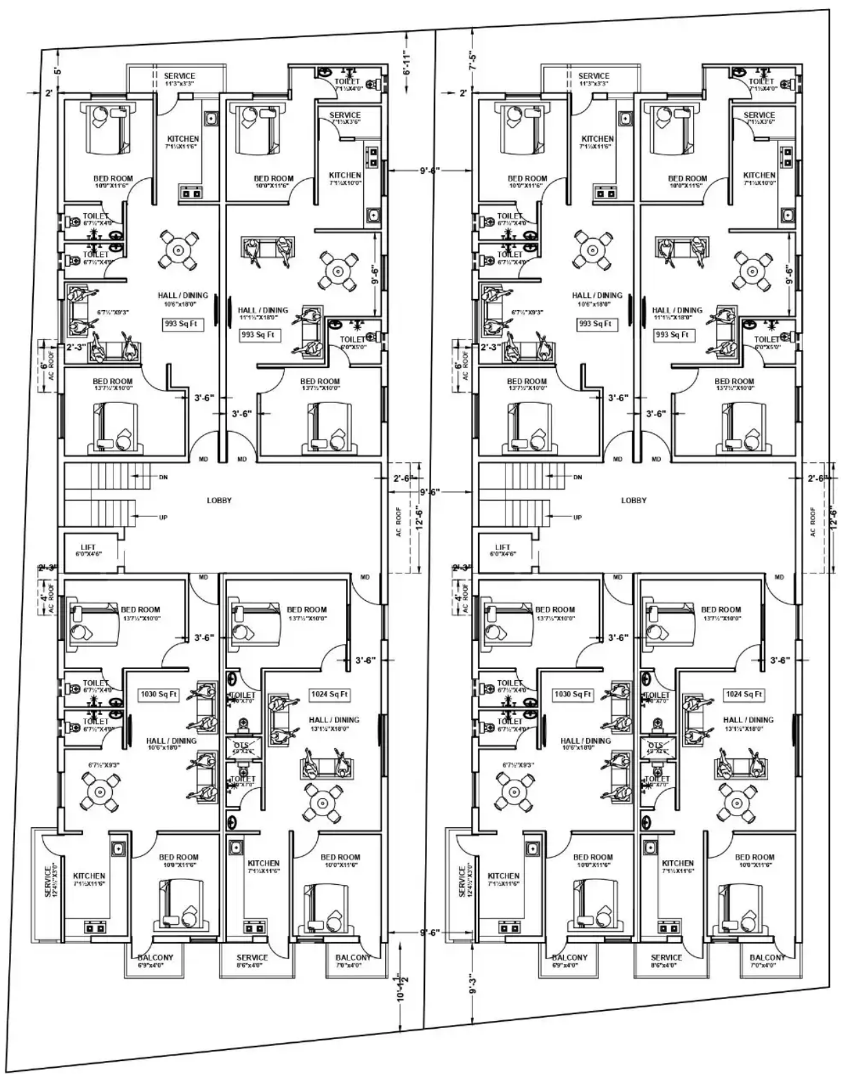
FIRST, SECOND & THIRD FLOOR PLAN
