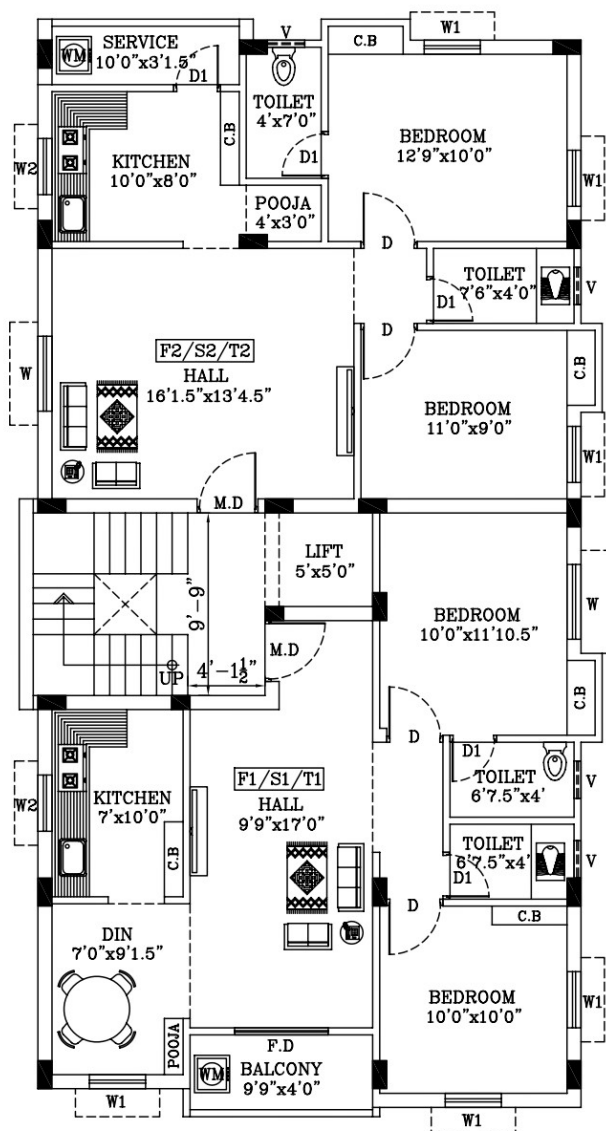
TYPICAL FLOOR PLAN (FIRST, SECOND & THIRD)
