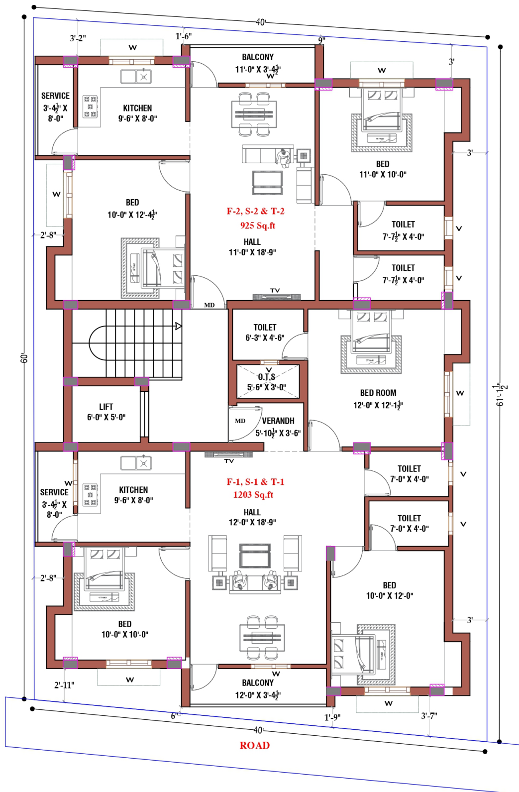
1ST, 2ND & 3RD FLOOR PLAN
