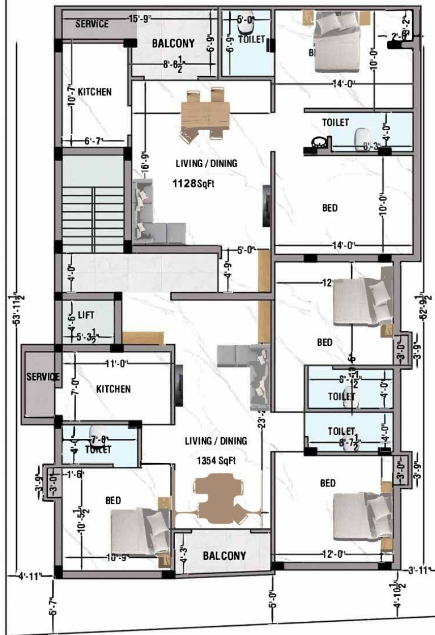
First, Second & Third Floor Plan
