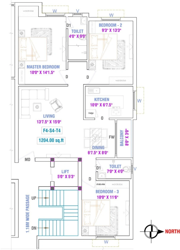
TYPICAL FLOOR PLAN (F1) FURNITURE LAYOUT ( FIRST, SECOND & THIRD ) F-4, S4, T4 : 1204.00 SQ.FT
