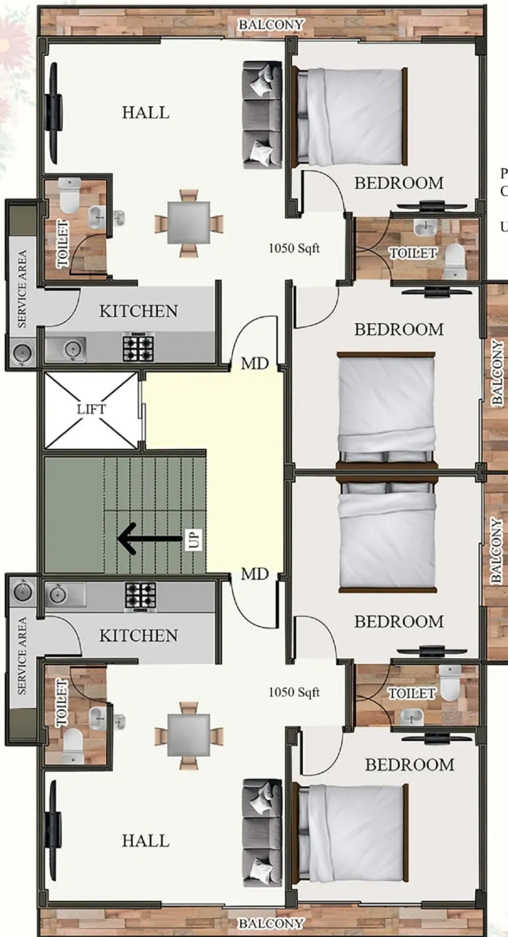
TYPICAL FLOOR PLAN [ FIRST, SECOND & THIRD]
