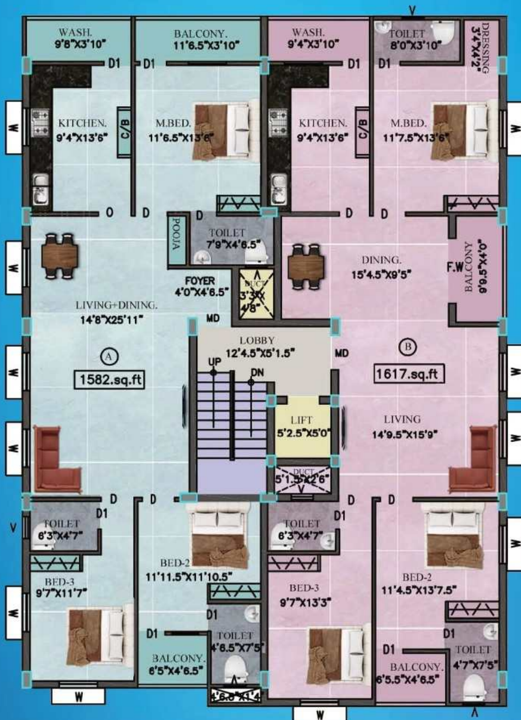
TYPICAL 1 st , 2 nd & 3 rd FLOOR PLAN
