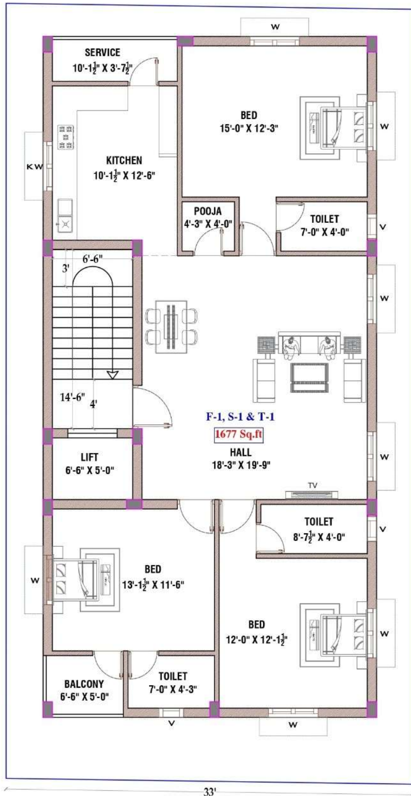
1st, 2nd AND 3rd FLOOR PLAN
