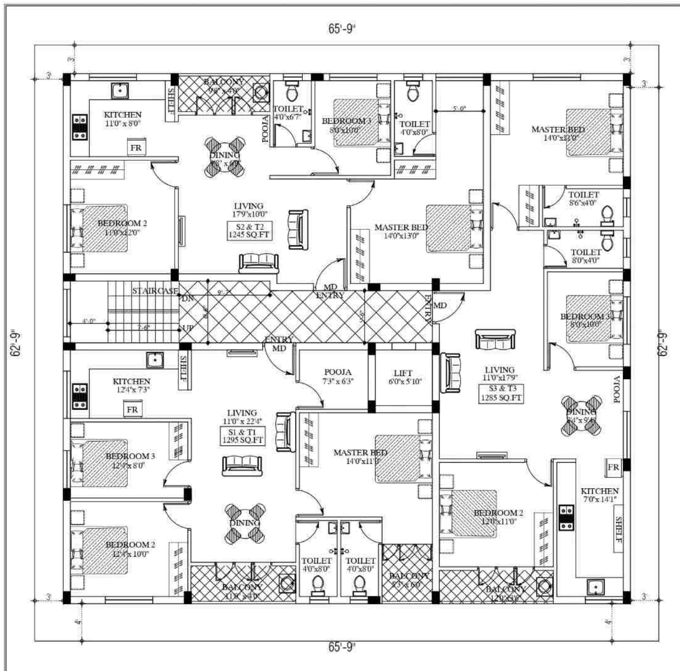
PLOT 5A AND 5B SECOND AND THIRD FLOOR PLAN
