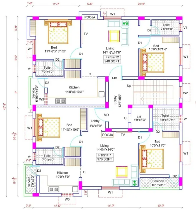
TYPICAL FLOOR PLAN FIRST, SECOND & THIRD FLOOR
