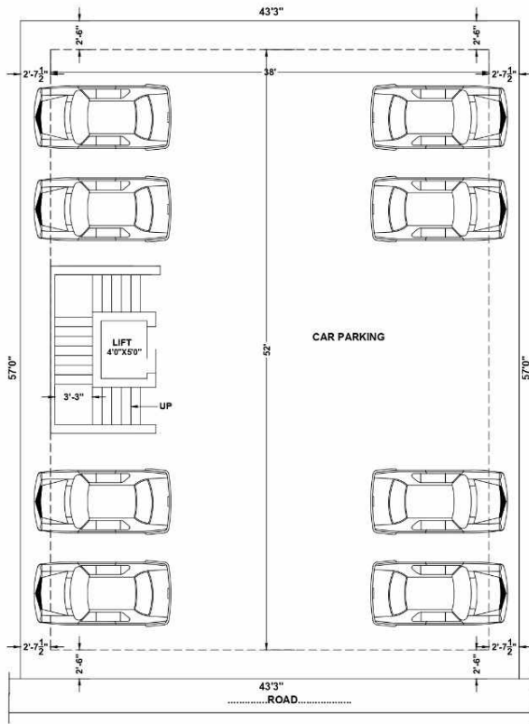
SITE CUM STILT FLOOR PLAN
