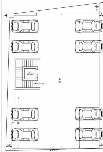
SITE CUM STILT FLOOR PLAN
