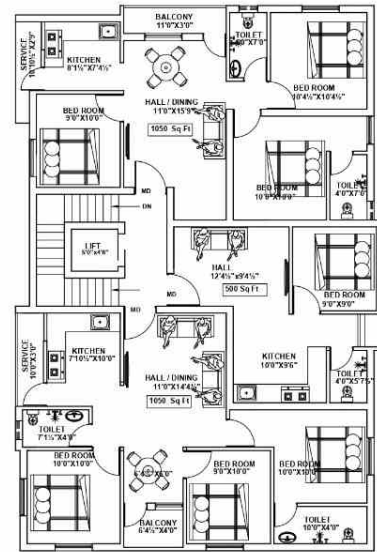
SECOND & THIRD FLOOR PLAN
