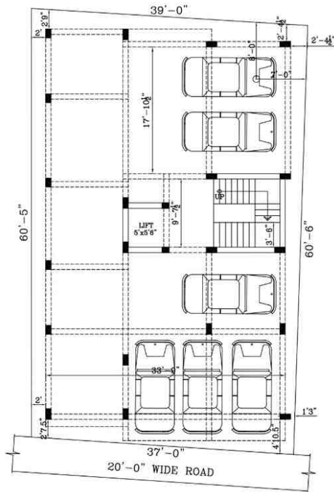
SITE CUM GROUND FLOOR PLAN
