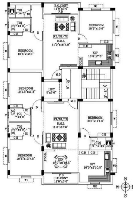
TYPICAL FLOOR PLAN (FIRST, SECOND & THIRD)
