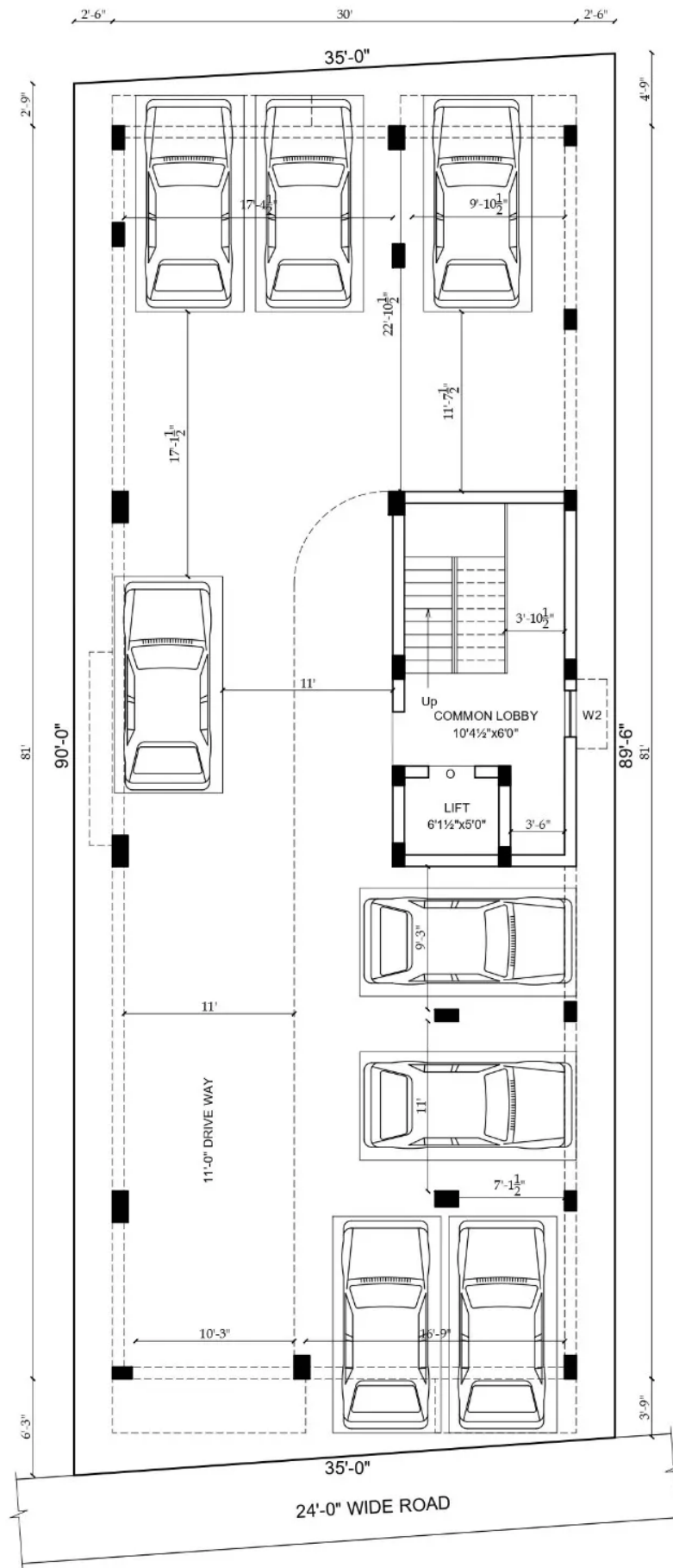
SITE CUM STILT FLOOR PLAN
