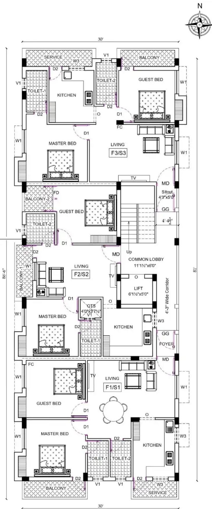
TYPICAL FLOOR PLAN FIRST & SECOND FLOOR
